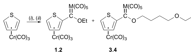
Scheme 2 (i) LiBu, thf, [\text{M}(\text{CO})_6] ; (ii) \text{Et}_3\text{OBF}_4 , \text{CH}_2\text{Cl}_2
